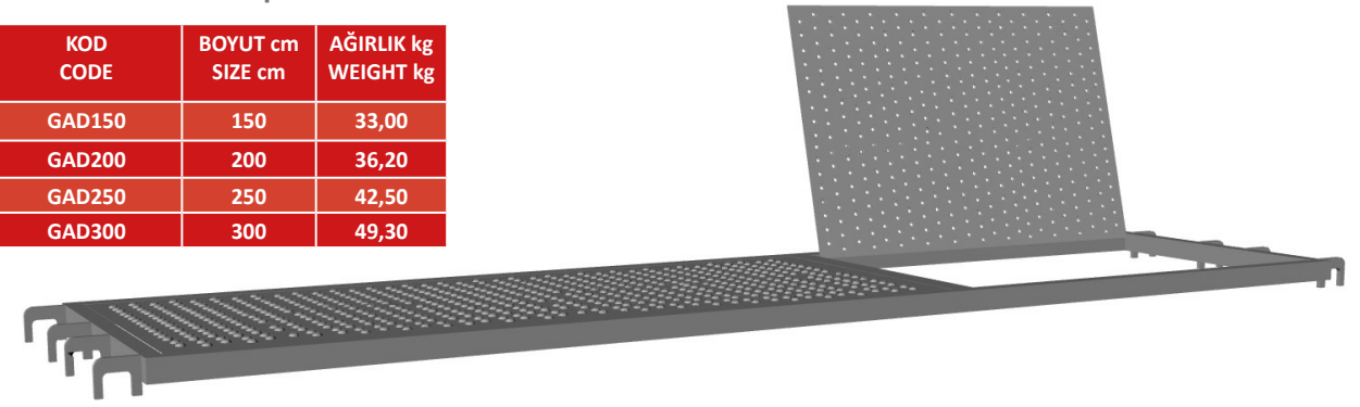
Kapaklı Kalaslı Metal Plank with Trapdoor
